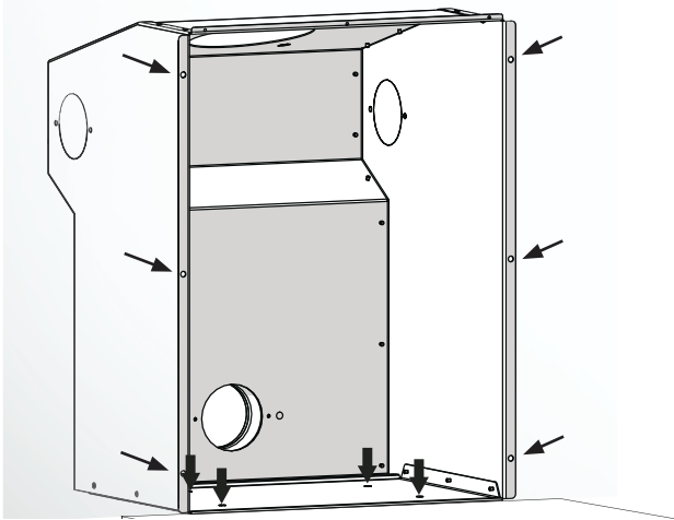
Fig. 16 Secure casing
