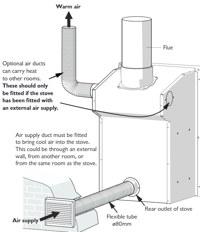
Fig. 12 Air supply
