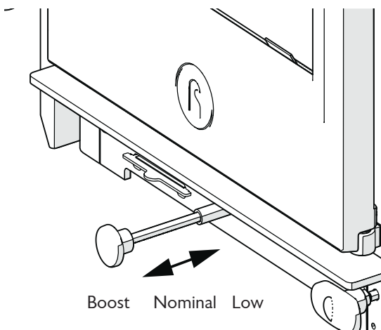
Fig. 3 Stove controls
