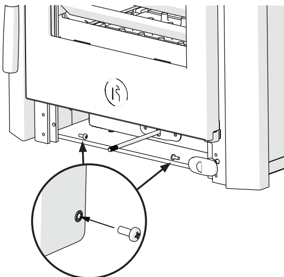
Fig. 21 Secure trim
