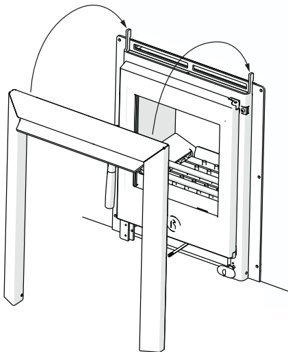
Fig. 20 Attach trim
