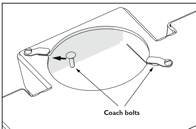
Fig. 17 Fit coach bolts
