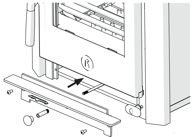
Fig. 22 Lower trim
