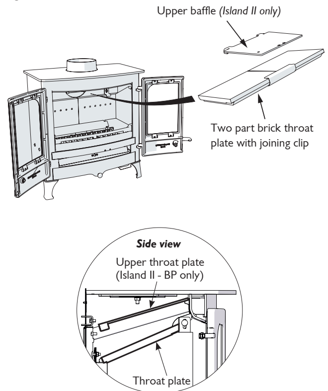
Fig.5 Throat Plate Location
